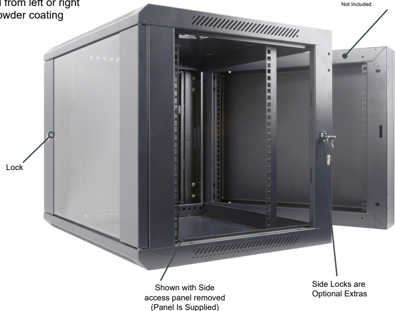
Wall Box Mount 100mm deep Powerboard Patchboard Not Included
